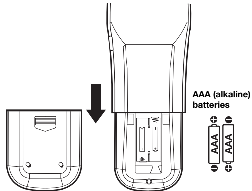
Figure 2. Installing batteries
